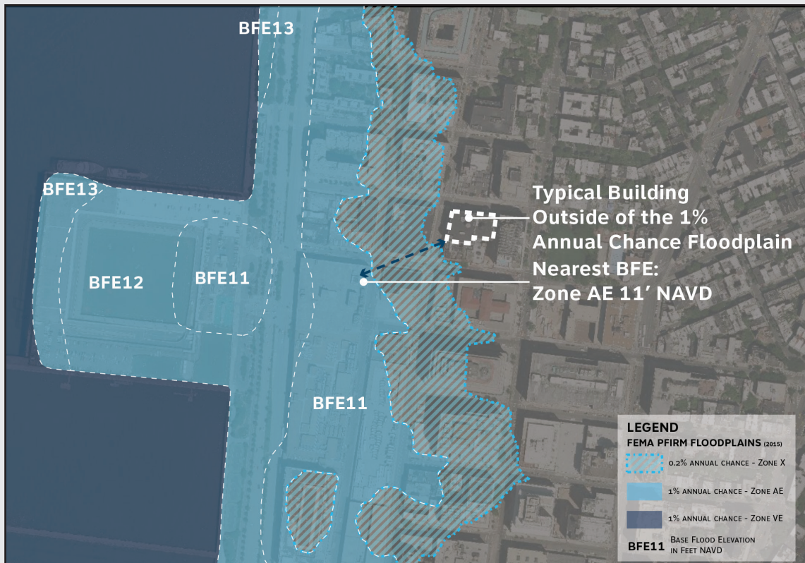
Figure 11 - This schematic map shows how to locate the nearest adjacent 1% floodplain elevation from a given project site.
