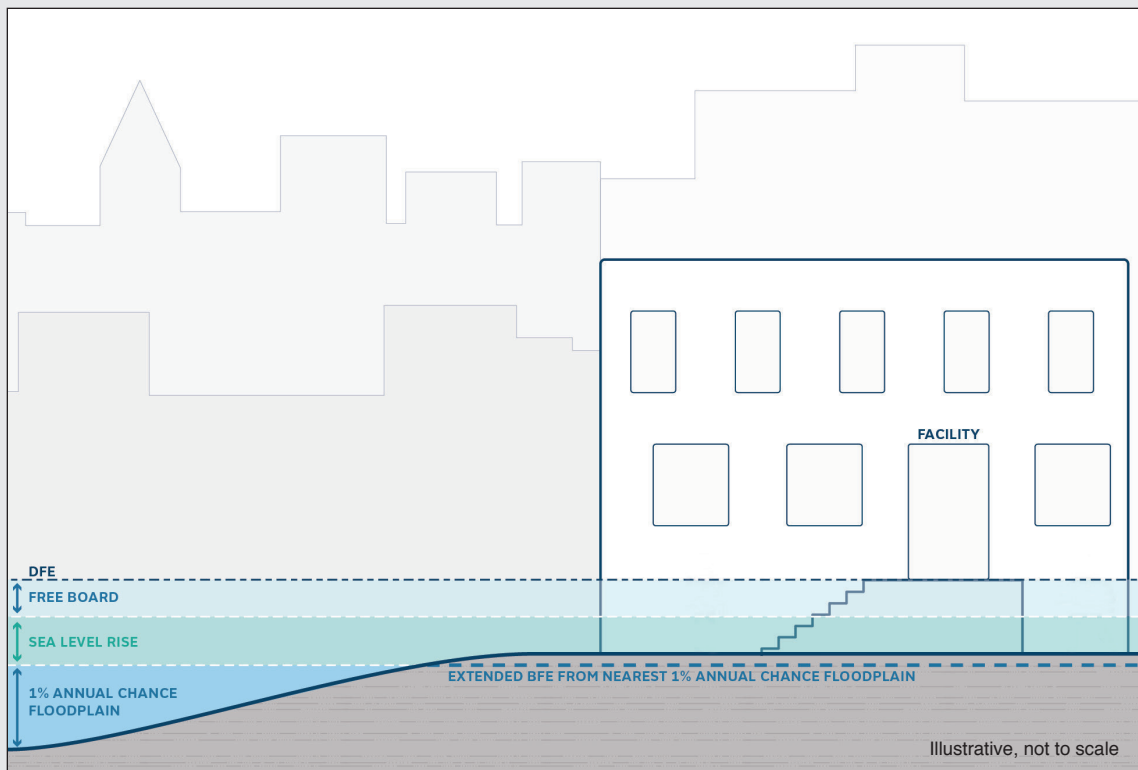
Figure 12 - This schematic shows how to use a base flood elevation in the current floodplain, with sea level rise and freeboard, added, to determine a design flood elevation for a facility located in the future floodplain.
