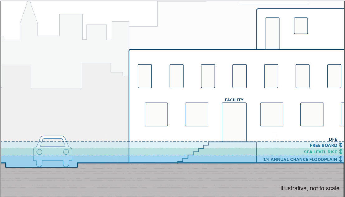
Figure 9 - This schematic shows how to determine the DFE of a facility within the current 1% floodplain.
