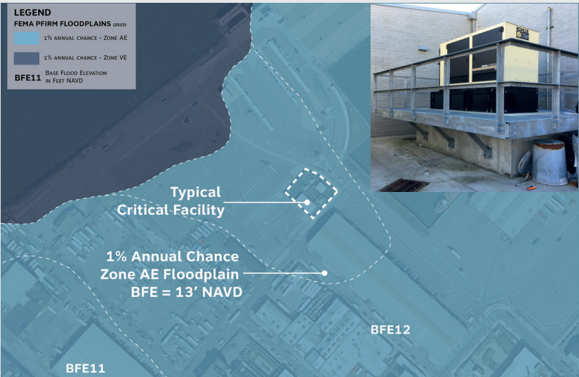
Figure 8 - Example of how to locate a facility within the current floodplain and determine the BFE. Inset: outdoor elevated emergency generator at the facility elevated to a sea level rise-adjusted DFE specific to its useful life.
