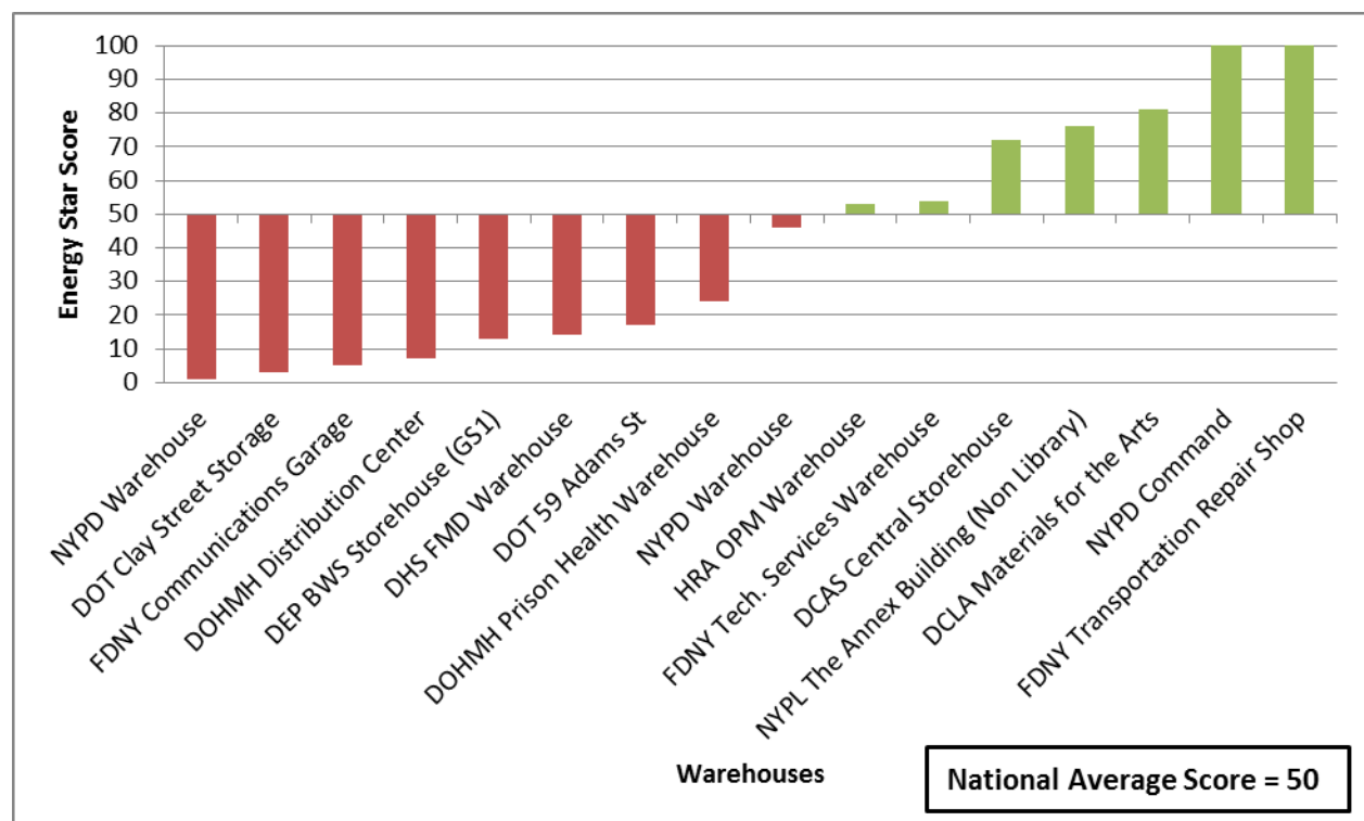
Figure 15: Non-Refrigerated Warehouse Benchmarking Results, 2010
