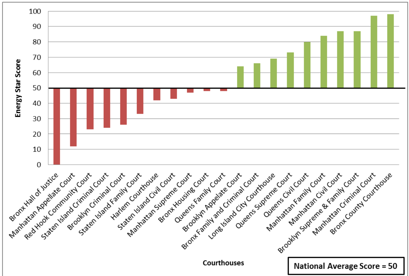
Figure 8: Courthouse Benchmarking Results, 2010
