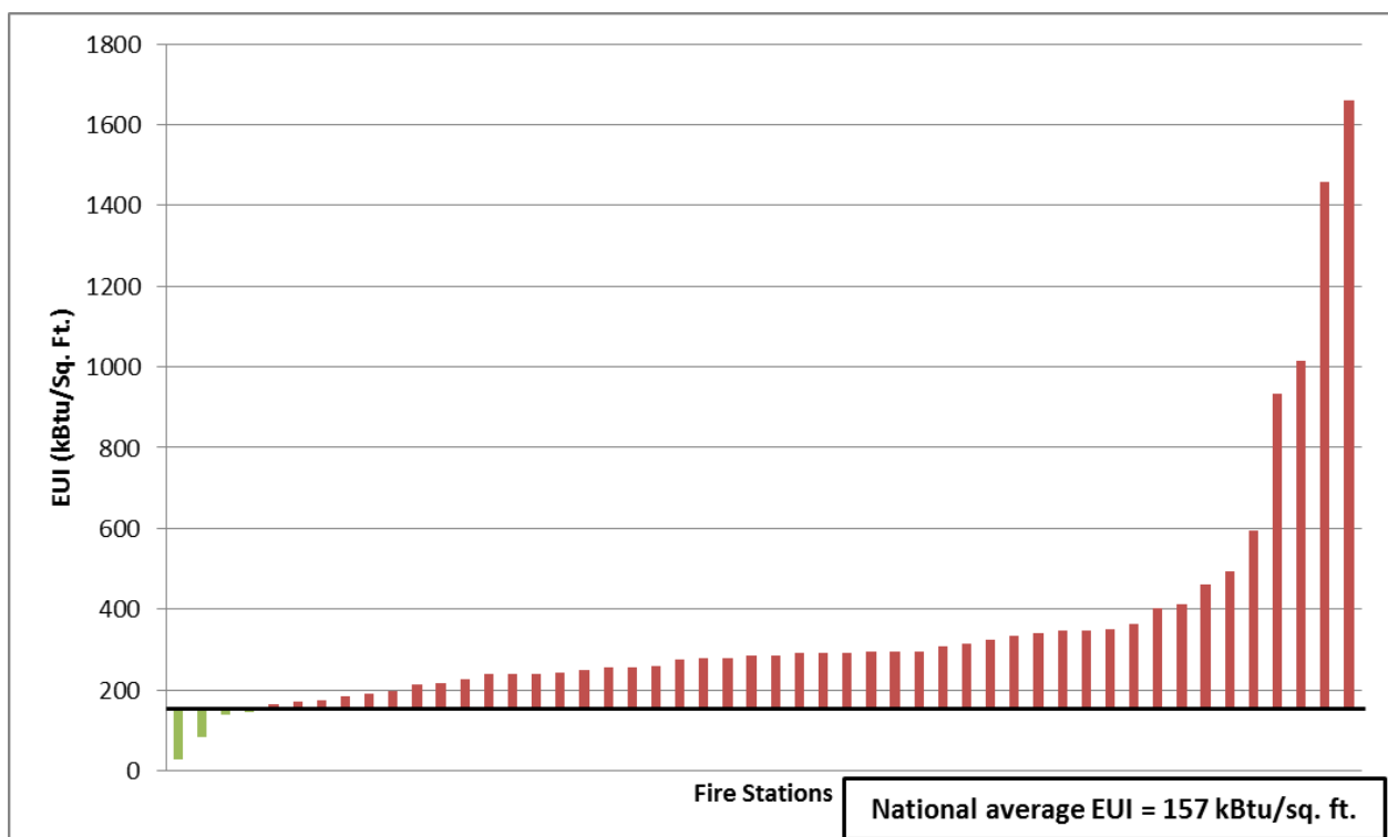
Figure 9: Fire Station EUI Results, 2010
