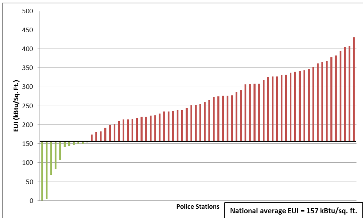
Figure 14: Police Station EUI Results, 2010
