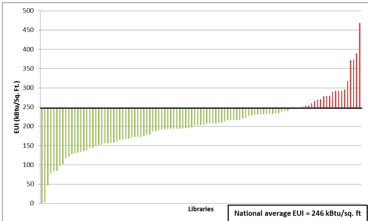
Figure 11: Library EUI Results, 2010
